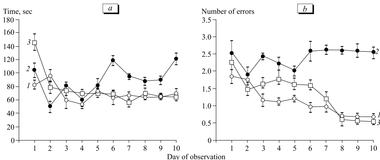
Fig. 1. Time of passing the maze ( a ) and number of errors (entrances into blind arms, b ) in experimental and controls rats exposed to toluene starting from the age of 25 days. Here and in Fig. 2: 1) control rats; 2) experimental rats tested immediately after termination of inhalations; 3) experimental rats tested in 90 days after the end of toluene inhalations.
